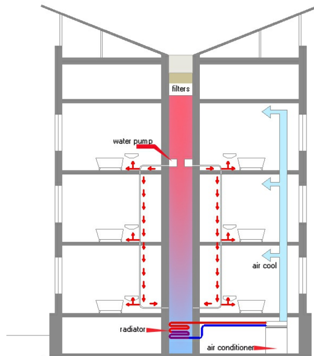
scheme using rainwater in hot water supply system
