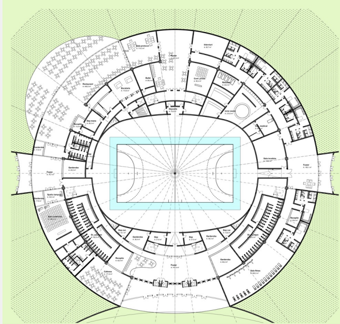
PLAN PARTER SC. 1/200
